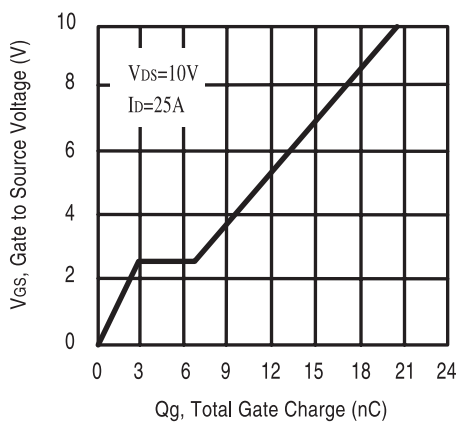
Figure 9. Gate Charge
